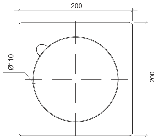
FD 015: Floor Drain with Removable Grid & securing Screws with Cover (3 pc set)
