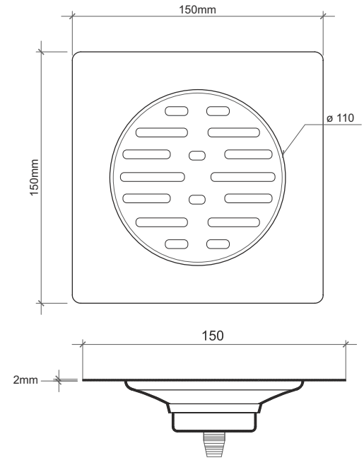
FD 012: Floor Drain
