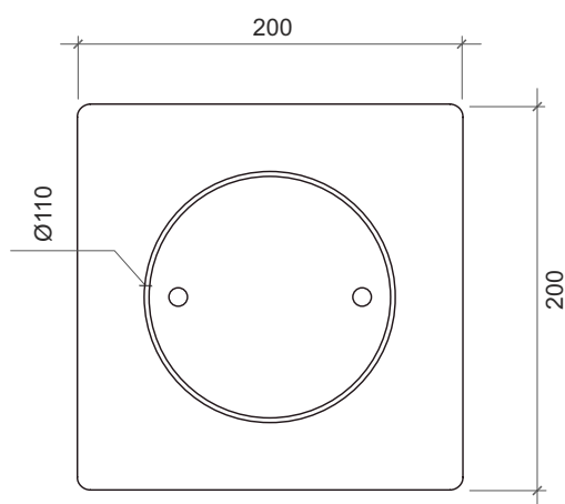
FD 016 : Floor Drain - Clean out Floor Drain with removable Cover and Securing Screws
