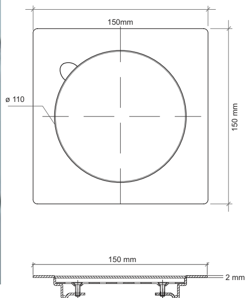
FD 011: Floor Drain with Removable Grid & securing Screws with Cover (3 pc set)
