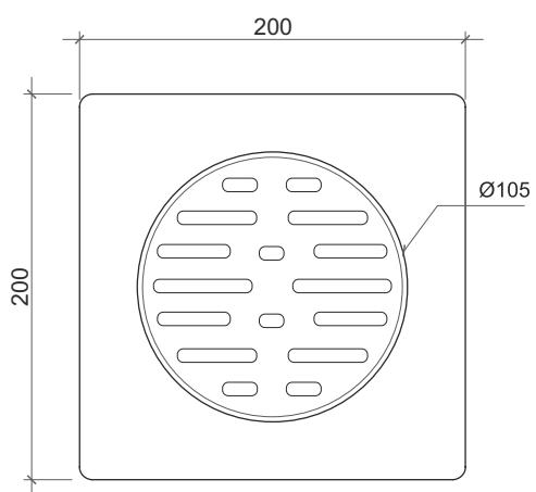
FD 014: Floor Drain
