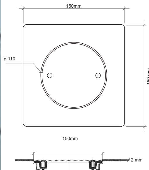
FD 013 : Floor Drain - Clean out Floor Drain with removable Cover and Securing Screws
